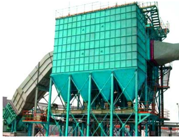
PULSE JET BAG FILTERS
